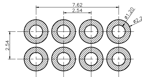
Recommended pcb layout layout tolerance: ±0.05mm
