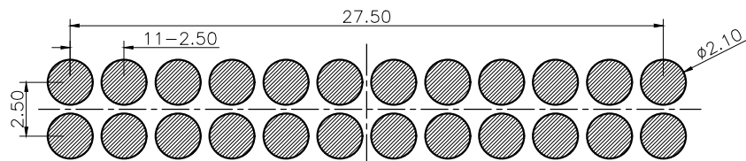
Recommended pcb layout Layout tolerance: ±0.05mm
