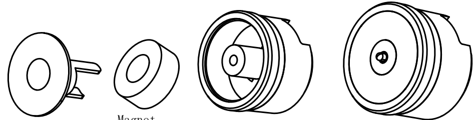
Shell .Salt Spray: 72 Hours Magnet .Salt Spray: 48 Hours Housing
