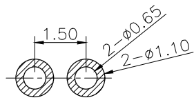
Recommended pcb layout Layout tolerance: ±0.05mm
